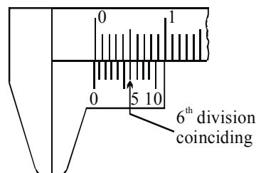
Negative zero error = (-0.04 cm) and its correction
